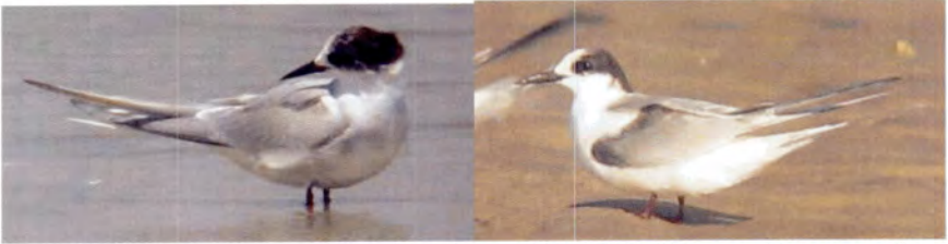
Figure H. Typical birds from 10 Jun 07 (left) and 16 Jun 07 (right, one of two present).
